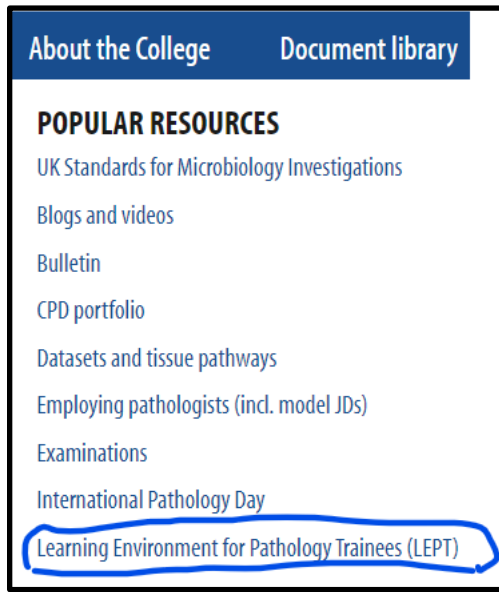
Screenshot 1
